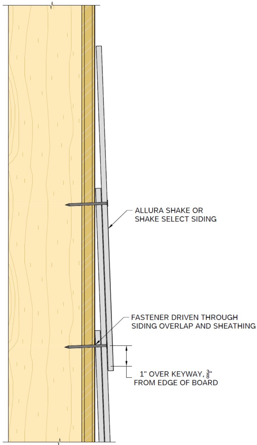
Figure 7 – Allura® and TerraPlank™ Shake and Allura® Shake Select General Installation
